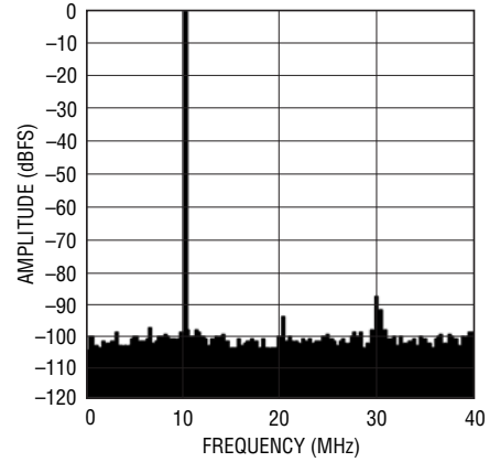
LTC2173-14: 8k Point FFT, f_{IN} = 70\text{MHz} -1\text{dBFS} , 80Msps
