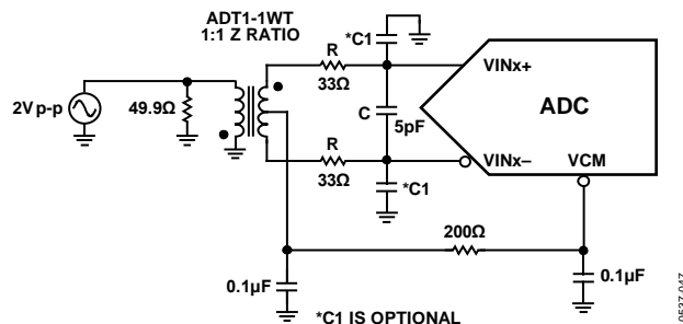
Figure 56. Differential Transformer-Coupled Configuration for Baseband Applications
