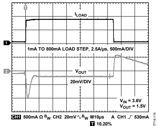
Figure 16. Load Transient Response, C_{IN} = 22 \mu F, C_{OUT} = 22 \mu F
