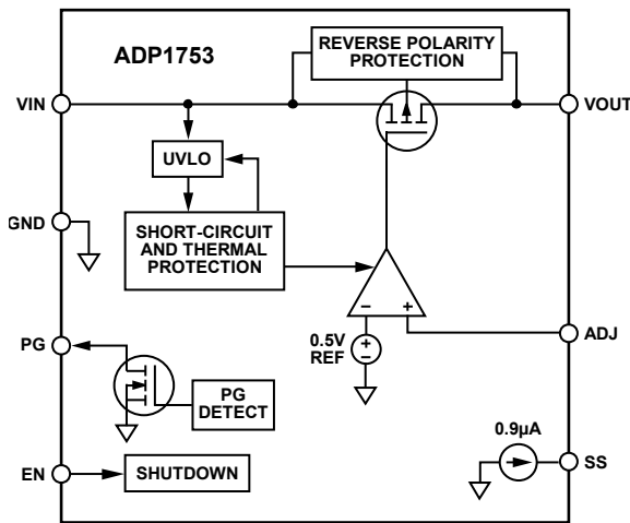
Figure 25. ADP1753 Internal Block Diagram
