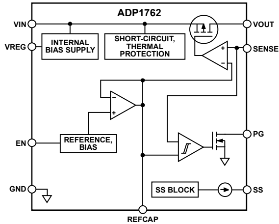
Figure 23. Functional Block Diagram, Fixed Output
