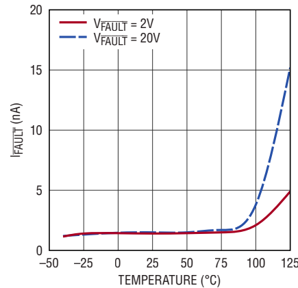
FAULT Pin Leakage Current
