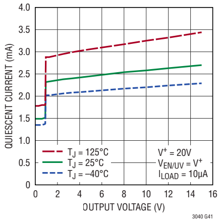
Quiescent Current
