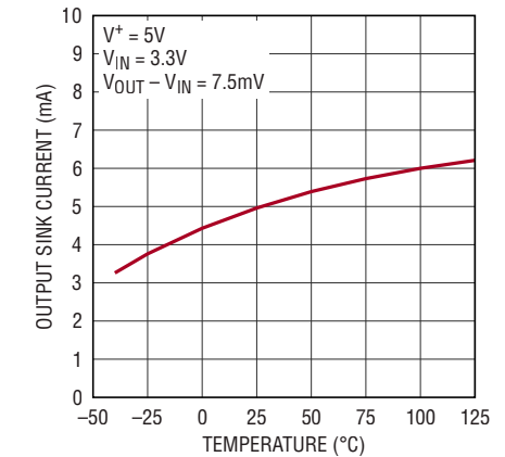
Output Overshoot Recovery Current Sink
