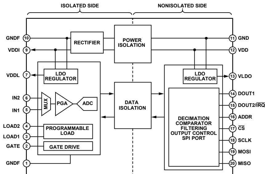
Figure 24. ADE1202 Nonisolated and Isolated Sides
