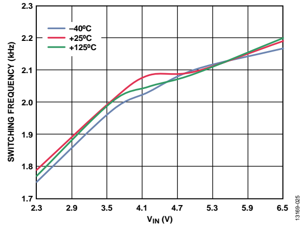
Figure 25. Switching Frequency vs. VIN
