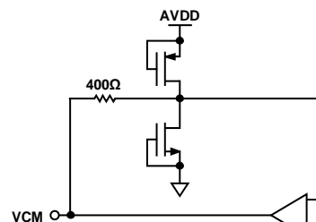
Figure 42. Equivalent VCM Circuit
