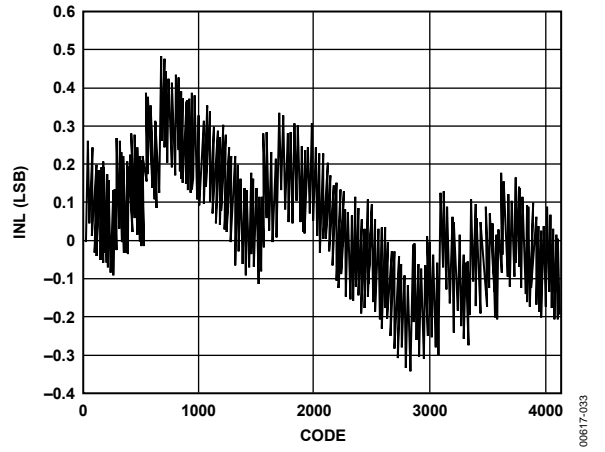
Figure 33. Typical INL
