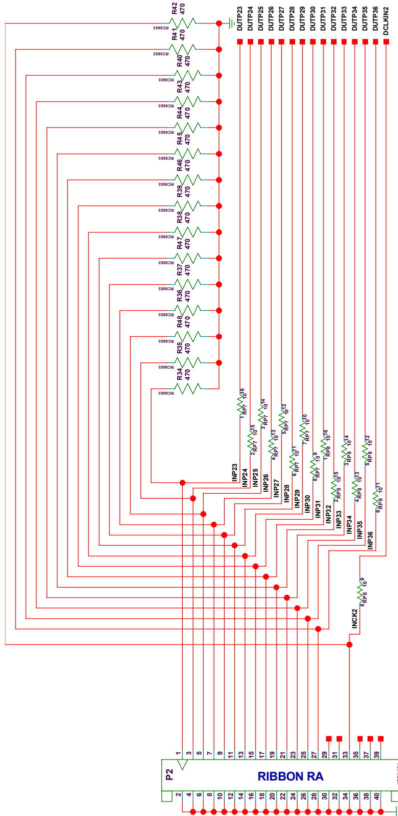
Figure 90. Digital Input Signaling (2)
