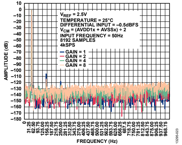
Figure 29. FFT Plot at 4kSPS, Low Power Mode, Input Frequency ( f_{IN} ) = 50 Hz, (This Plot is a Close Up Perspective of the Original Data)
