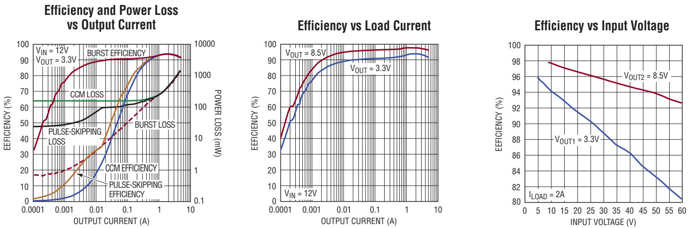
Figure 13. High Efficiency Dual 8.5V/3.3V Step-Down Converter
