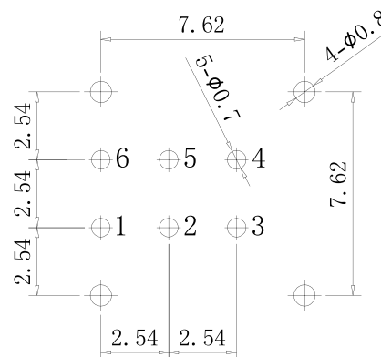
B-B PCB cut-outs
