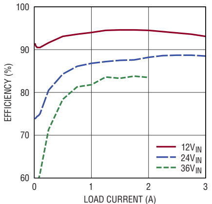
Efficiency, V_{OUT} = 8\text{V} , BIAS = 5V
