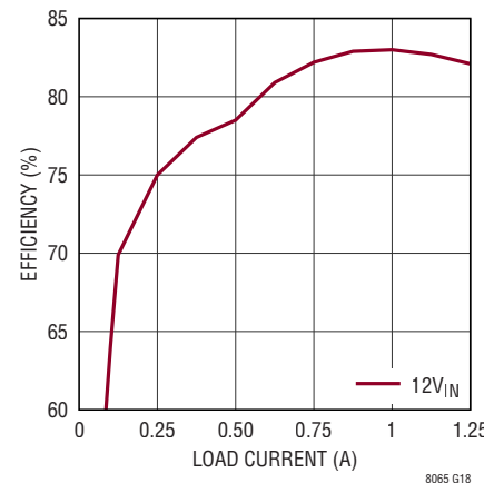
Efficiency, V_{OUT} = -18\text{V} , BIAS tied to LTM8065 GND
