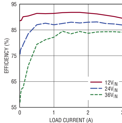
Efficiency, V_{OUT} = 5\text{V} , BIAS = 5V
