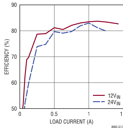
Efficiency, V_{OUT} = -15\text{V} , BIAS tied to LTM8065 GND
