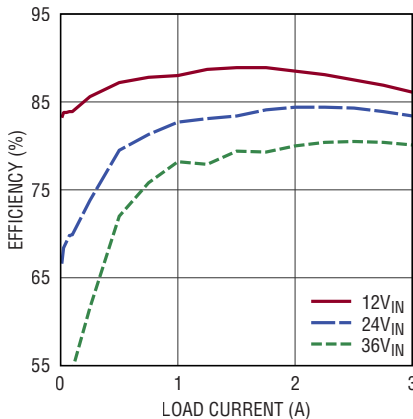
Efficiency, V_{OUT} = 3.3\text{V} , BIAS = 5V
