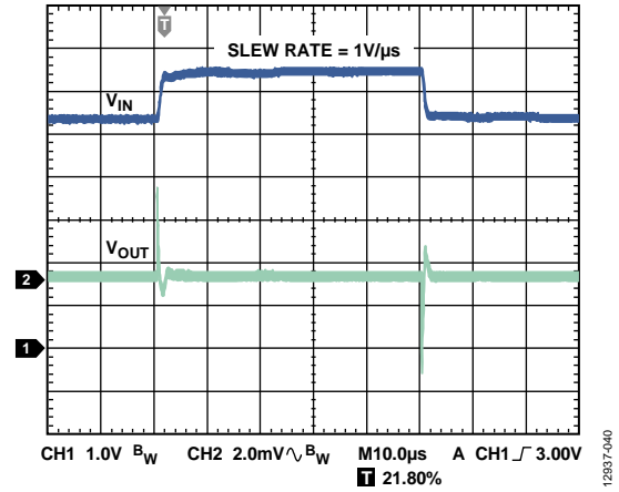
Figure 38. Line Transient Response, 1 V Input Step, I_{LOAD} = 1.2 \text{ A} , V_{OUT} = 1.8 \text{ V} , V_{IN} = 2.5 \text{ V} , Channel 1 = V_{IN} , Channel 2 = V_{OUT}
