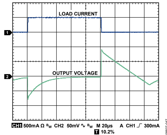
Figure 52. Load Transient Response, C_{IN}, C_{OUT} = 1\ \mu\text{F} , I_{LOAD} = 1\text{ mA to } 500\text{ mA} , V_{OUT} = 5\text{ V} , V_{IN} = 7\text{ V}
