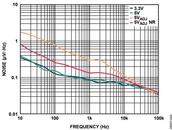
Figure 49. Output Noise Spectral Density, I_{LOAD} = 10\text{ mA} , C_{OUT} = 1\ \mu\text{F}
