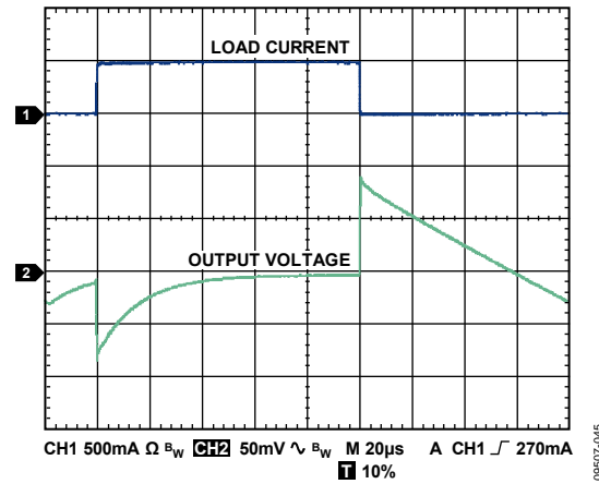
Figure 50. Load Transient Response, C_{IN}, C_{OUT} = 1\ \mu\text{F} , I_{LOAD} = 1\text{ mA to } 500\text{ mA} , V_{OUT} = 1.8\text{ V} , V_{IN} = 5\text{ V}
