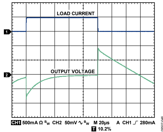
Figure 51. Load Transient Response, C_{IN}, C_{OUT} = 1\ \mu\text{F} , I_{LOAD} = 1\text{ mA to } 500\text{ mA} , V_{OUT} = 3.3\text{ V} , V_{IN} = 5\text{ V}
