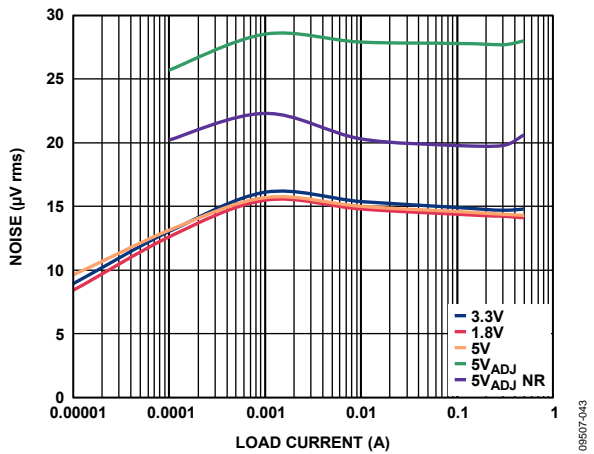
Figure 48. Output Noise vs. Load Current and Output Voltage, C_{OUT} = 1\ \mu\text{F}
