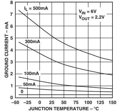
TPC 6. Ground Current vs. Junction Temperature
