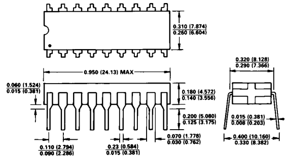
18-Pin Cerdip (Suffix Q)
