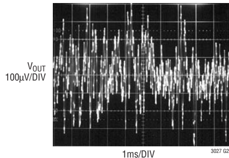
10Hz to 100kHz Output Noise C BYP = 0
