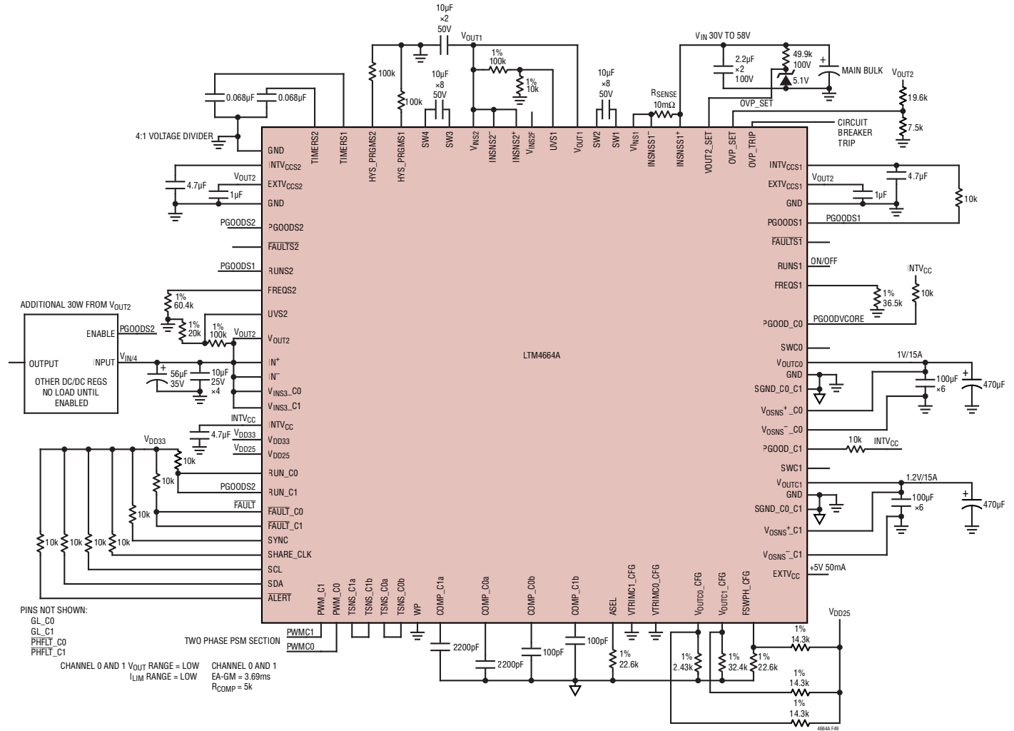
Figure 49. 30V – 58V to 1V and 1.2V at 15A, with Additional 30W from V OUT2 . Integrated Power System Management Features Accessible Over 2-Wire I 2 C/SMBus/PMBus Serial Interface. For Evaluation and More Information, See Demo Boards DC2143
