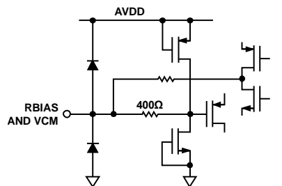
Figure 48. Equivalent RBIAS and VCM Circuit
