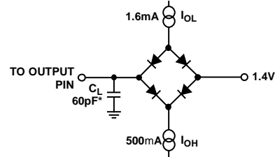
*IN SERIAL INTERFACE MODES, THE SYNC, SCLK, AND SDOOUT TIMINGS ARE DEFINED WITH A MAXIMUM LOAD C_L OF 10pF; OTHERWISE, THE LOAD IS 60pF MAXIMUM.
