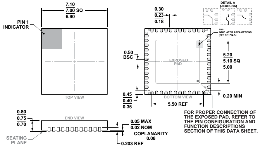
Figure 7. 48-Lead Lead Frame Chip Scale Package [LFCSP] 7 mm x 7 mm Body and 0.75 mm Package Height (CP-48-4)
