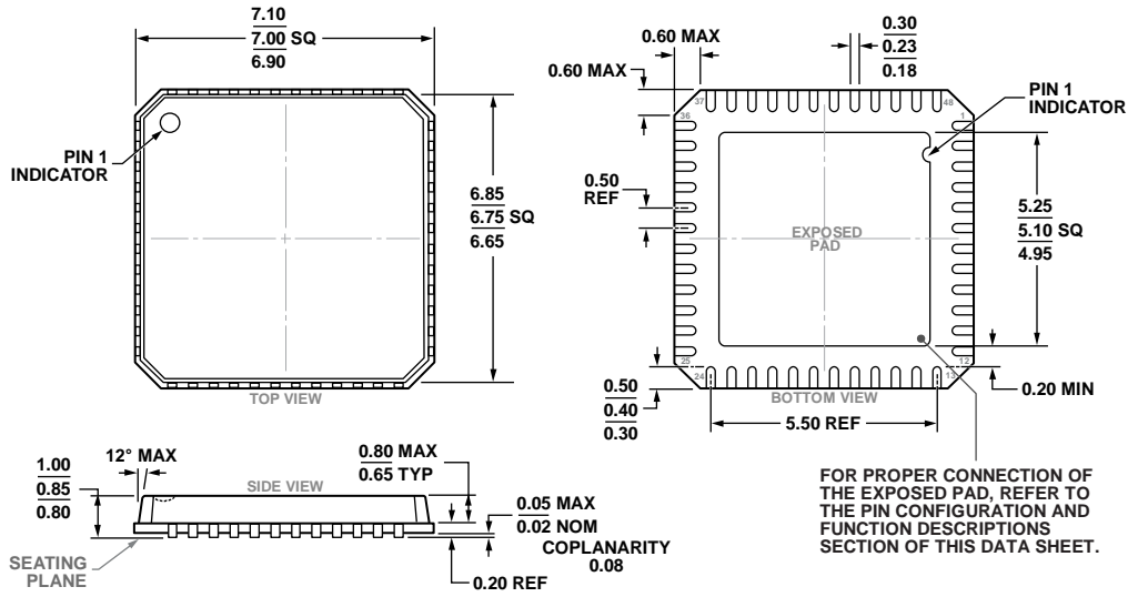
Figure 6. 48-Lead Lead Frame Chip Scale Package [LFCSP] 7 mm x 7 mm Body and 0.85 mm Package Height (CP-48-1)
