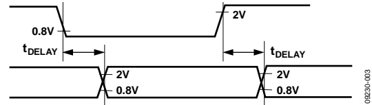
Figure 3. Voltage Reference Levels for Timing
