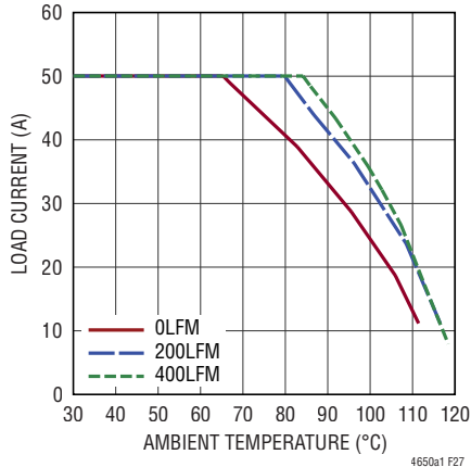
Figure 27. 5V to 1.8V Derating Curve, BGA Heat Sink
