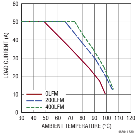
Figure 30. 12V to 3.3V Derating Curve, BGA Heat Sink
