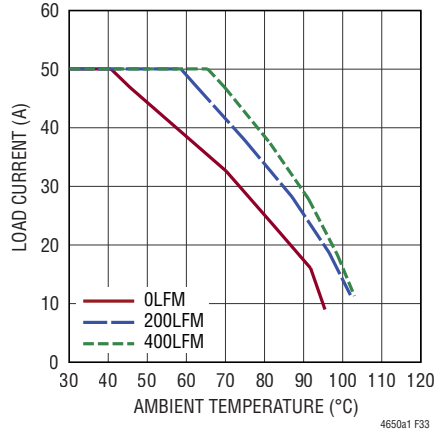
Figure 33. 12V to 5V Derating Curve, BGA Heat Sink
