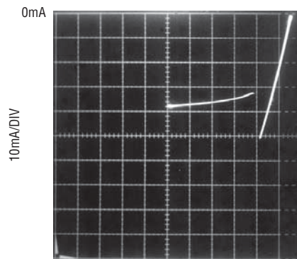
Short-Circuit Output Current vs V_{OUT} (Sourcing)
