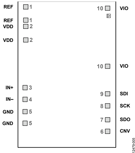
Figure 4. Pad Configuration
