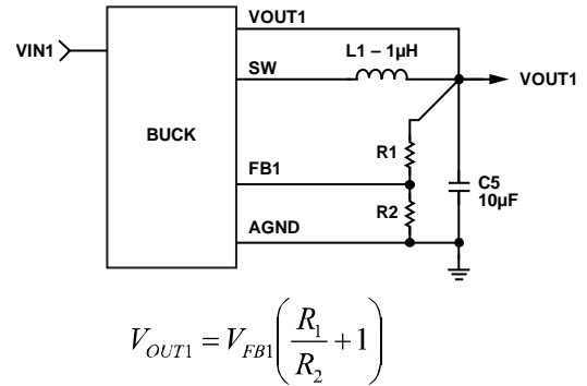
Figure 102. Buck External Output Voltage Setting
