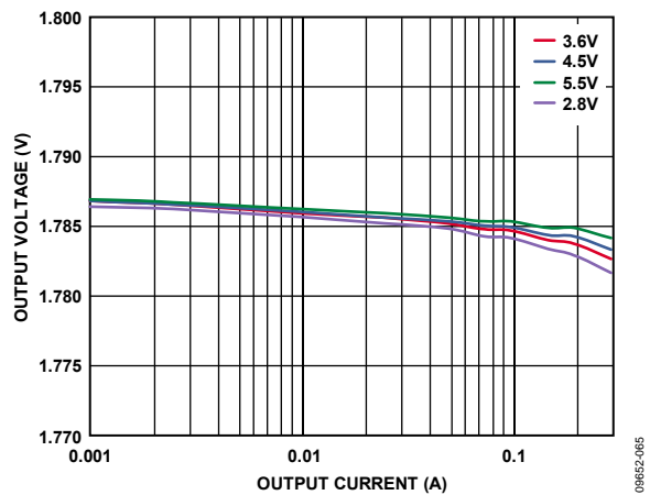
Figure 65. LDO1, LDO2 Load Regulation Across Input Voltage, V_{OUT} = 1.8 V
