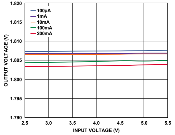
Figure 72. LDO1, LDO2 Line Regulation Across Input Voltage, V_{OUT} = 1.8 V
