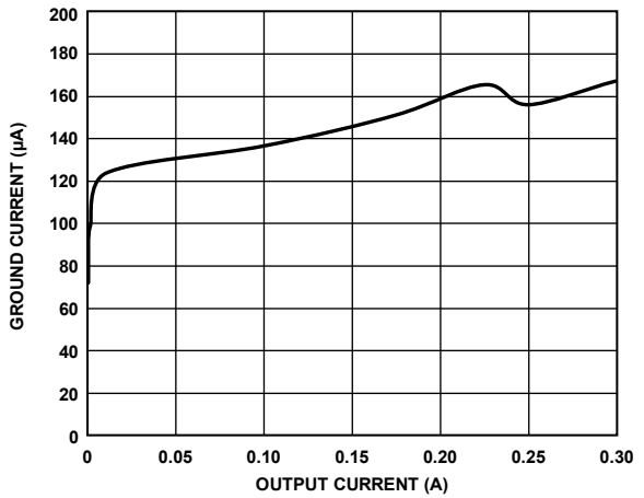
Figure 74. LDO1, LDO2 Ground Current vs. Output Current, V_{OUT} = 3.3 V
