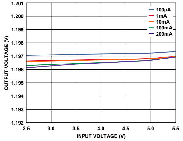
Figure 73. LDO1, LDO2 Line Regulation Across Input Voltage, V_{OUT} = 1.2 V
