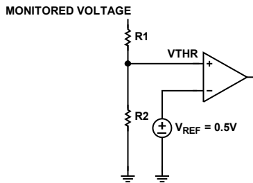
Figure 105. External Reset Threshold Programming
