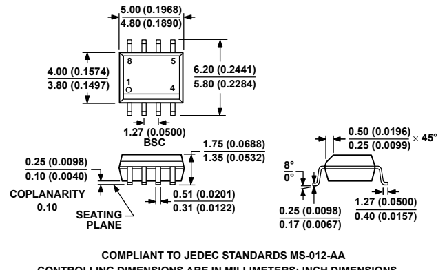
Figure 45. 8-Lead Standard Small Outline Package [SOIC_N] Narrow Body (R-8) Dimensions shown in millimeters and (inches)
