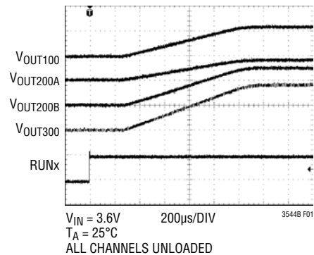
Figure 1. Regulator Soft-Start
