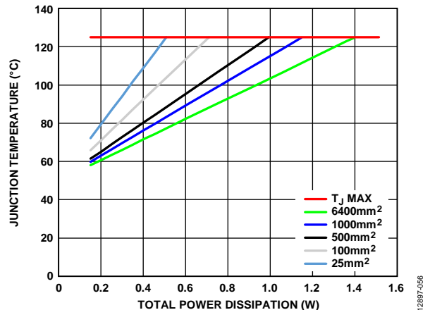
Figure 51. Junction Temperature vs. Total Power Dissipation, T_A = 50^\circ\text{C}
