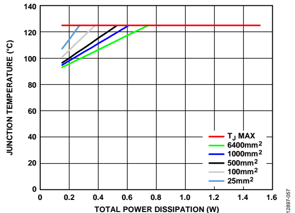
Figure 52. Junction Temperature vs. Total Power Dissipation, T_A = 85^\circ\text{C}
