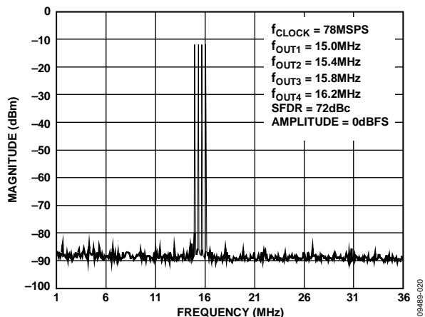
Figure 20. Four-Tone SFDR
