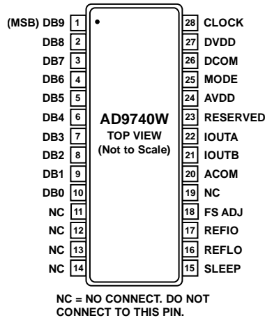
Figure 3. Pin Configuration
