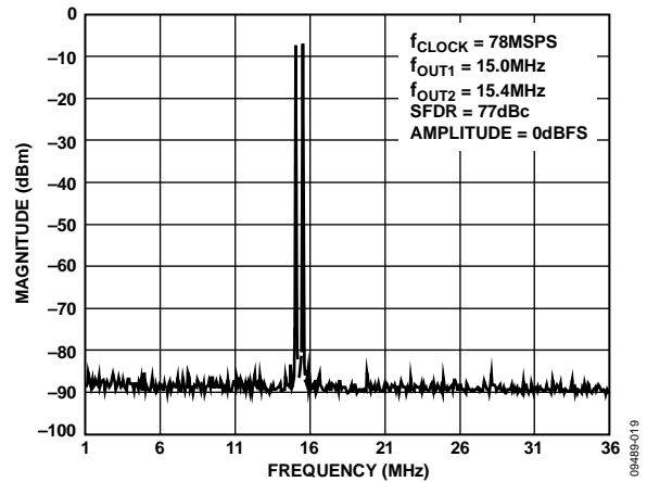
Figure 19. Dual-Tone SFDR
