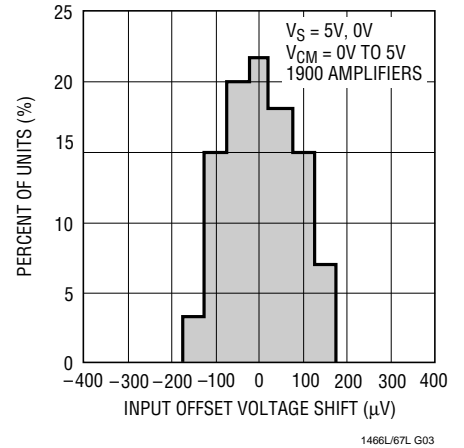
V OS Shift, V CM = 0V to 5V
