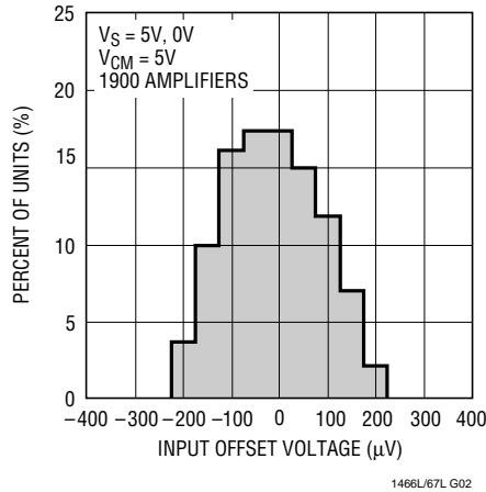
V OS Distribution, V CM = 5V
