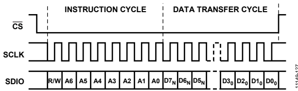
Figure 122. Serial Register Interface Timing, MSB-First Write
