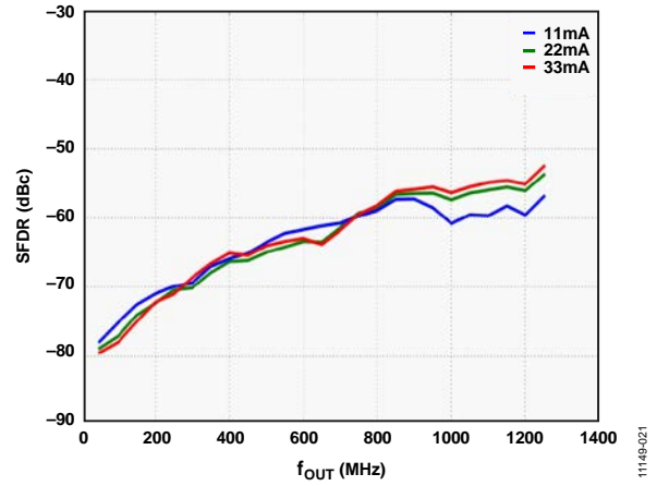
Figure 18. SFDR vs. f_{OUT} over DAC I_{OUTFS}
