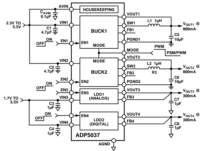
Figure 52. ADP5037 Fixed Output Voltages with Enable Pins
