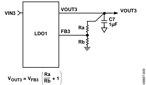
Figure 48. LDO1 External Output Voltage Setting
