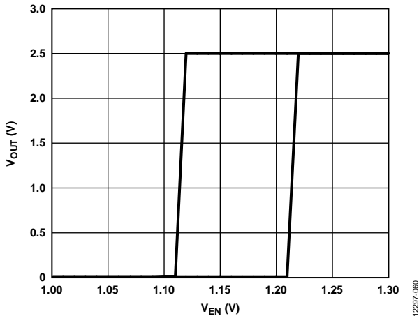
Figure 58. Typical V OUT Response to EN Pin Operation
