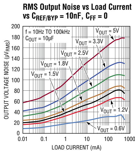
10Hz to 100kHz Output Noise C_{REF/BYP} = 10\text{nF} , C_{FF} = 0
