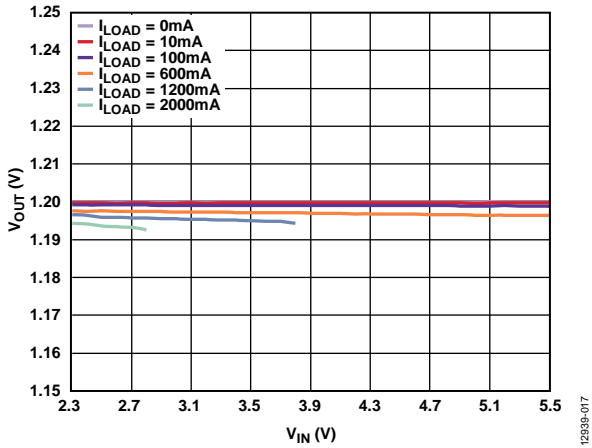
Figure 17. Output Voltage ( V_{OUT} ) vs. Input Voltage ( V_{IN} ) at Various Loads, V_{OUT} = 1.2 V
