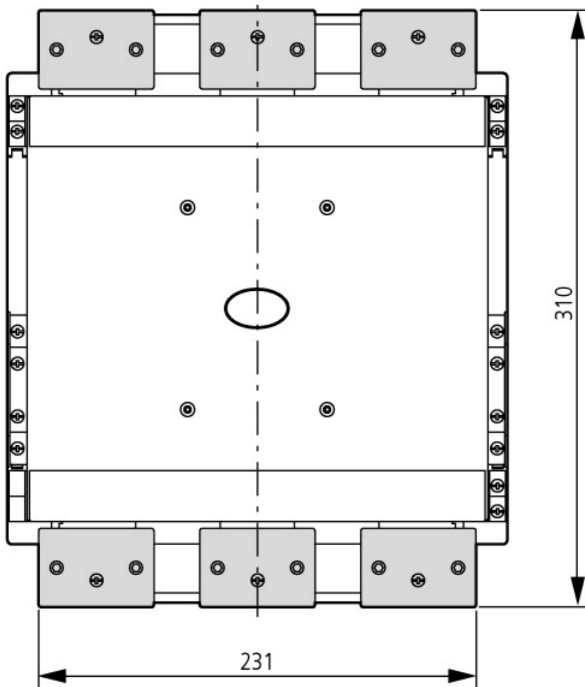
DILM580 ... DILM820
