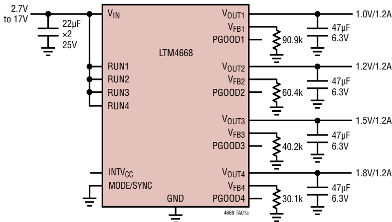
2.7V to 17V Input, Quad 1.0V, 1.2V, 1.5V, 1.8V Output DC/DC \mu Module Regulator
