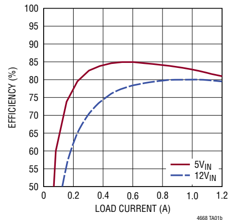
1.5V Output Efficiency (Each Channel)
