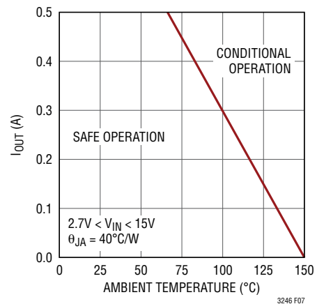
Figure 7. 3.3V Output Operation vs Ambient Temperature
