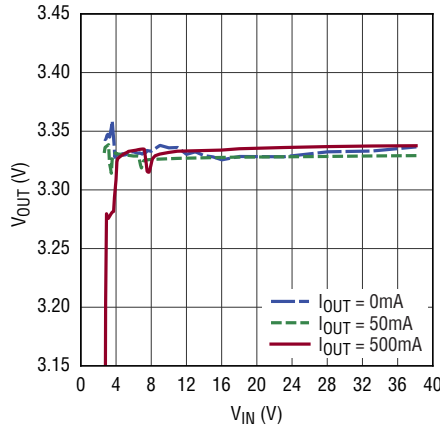
3.3V Fixed Output Voltage vs Input Voltage
