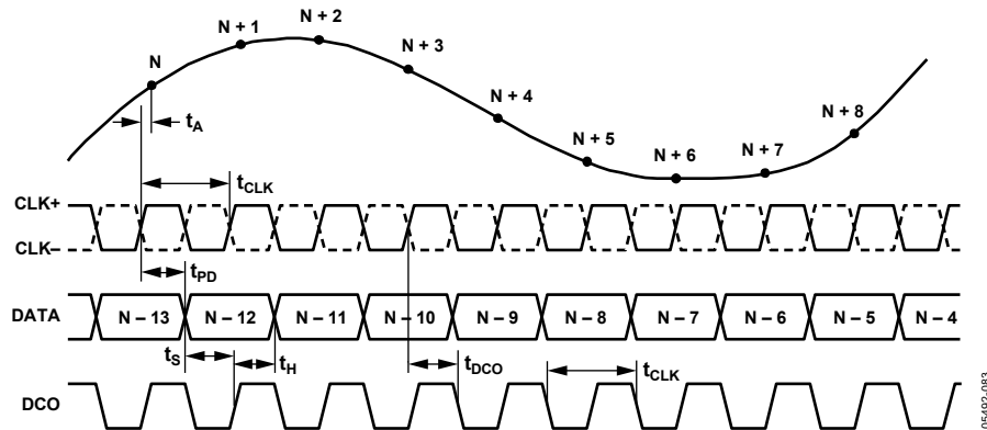
Figure 2. Timing Diagram
