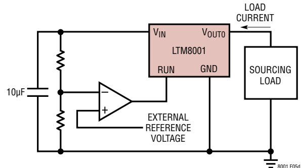
(5d) This Comparator Circuit Turns Off the LTM8001 if the Input Rises Above a Predetermined Threshold. When the LTM8001 Turns Off, the Energy Stored in the Internal Inductor Will Raise V_{IN} a Small Amount Above the Threshold.
