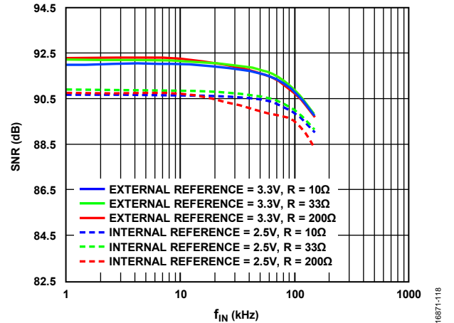
Figure 18. SNR vs. f_{IN} (R Means Resistance)
