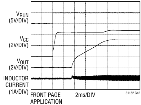
Soft-Start Waveforms
