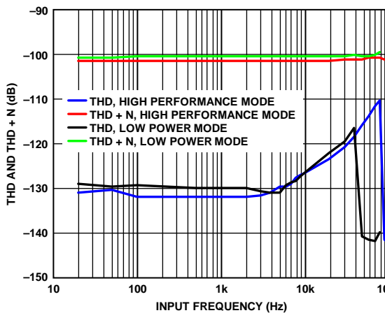
Figure 19. THD and THD + N vs. Input Frequency, -6 dBFS Input, 0.433 \times \text{ODR} Filter
