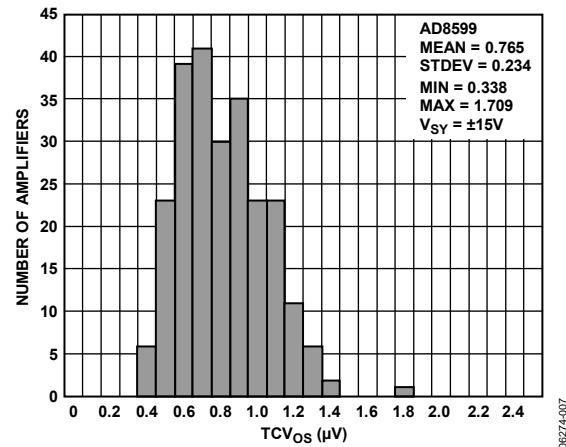
Figure 8. TCV 0s Distribution, -40°C ≤ T A ≤ +125°C
