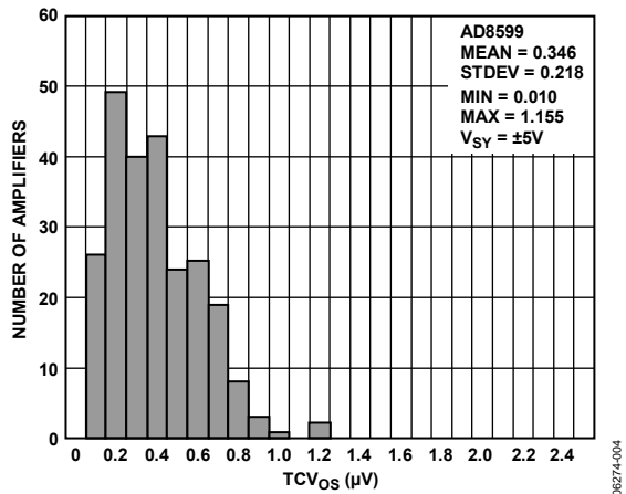
Figure 5. TCV 0s Distribution, -40°C ≤ T A ≤ +125°C
