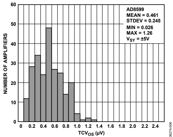
Figure 6. TCV 0s Distribution, -40°C ≤ T A ≤ +85°C
