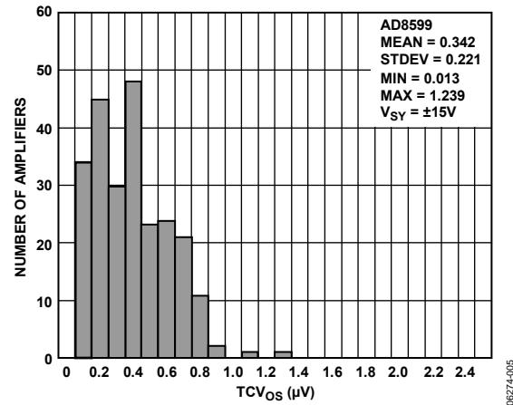
Figure 9. TCV 0s Distribution, -40°C ≤ T A ≤ +85°C
