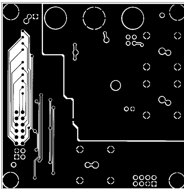
Figure 13d. Suggested Evaluation Circuit Board Solder Side Layout
