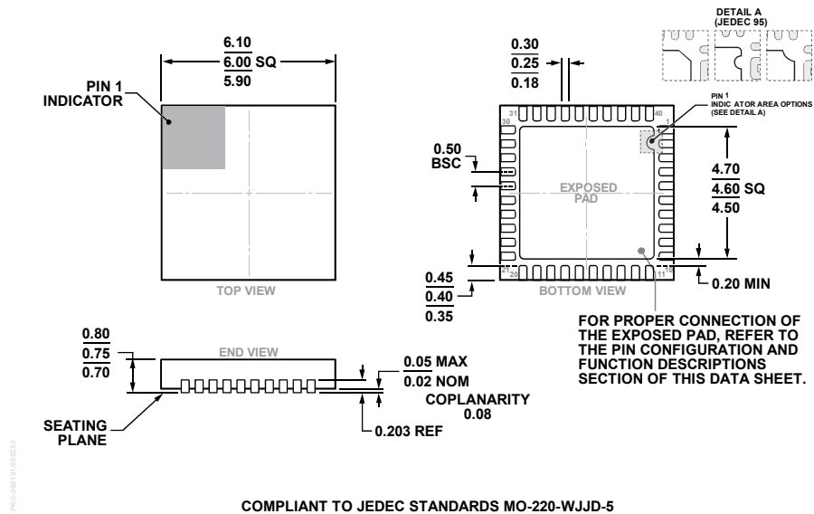
COMPLIANT TO JEDEC STANDARDS MO-220-WJJD-5 Figure 77. 40-Lead Lead Frame Chip Scale Package [LFCSP] 6 mm x 6 mm and 0.75 mm Package Height (CP-40-7) Dimensions shown in millimeters
