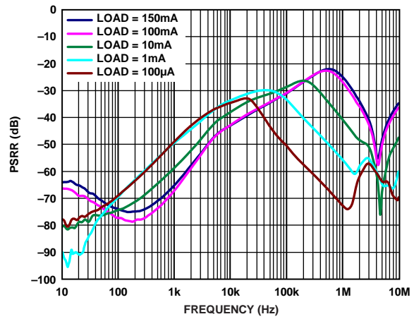
Figure 19. Power Supply Rejection Ratio (PSRR) vs. Frequency, Various Load Currents, V_{OUT} = 1.2\text{ V} , V_{IN} = 2.2\text{ V}
