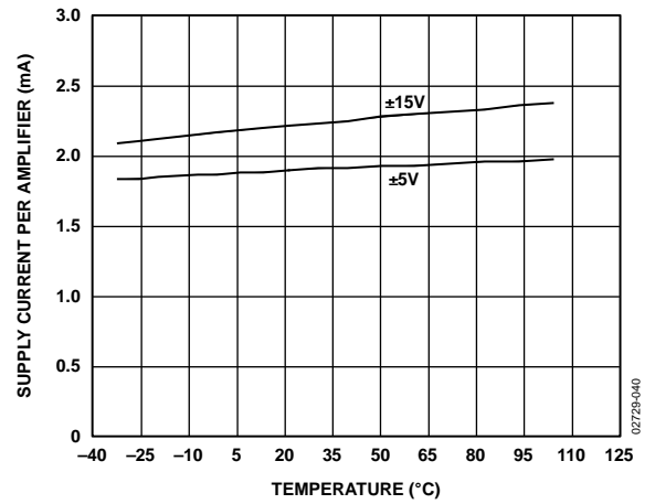
Figure 39. AD8513 Supply Current per Amplifier vs. Temperature
