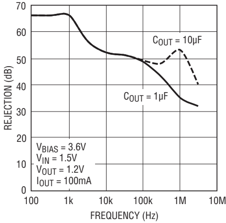
V_{IN} Ripple Rejection vs Frequency
