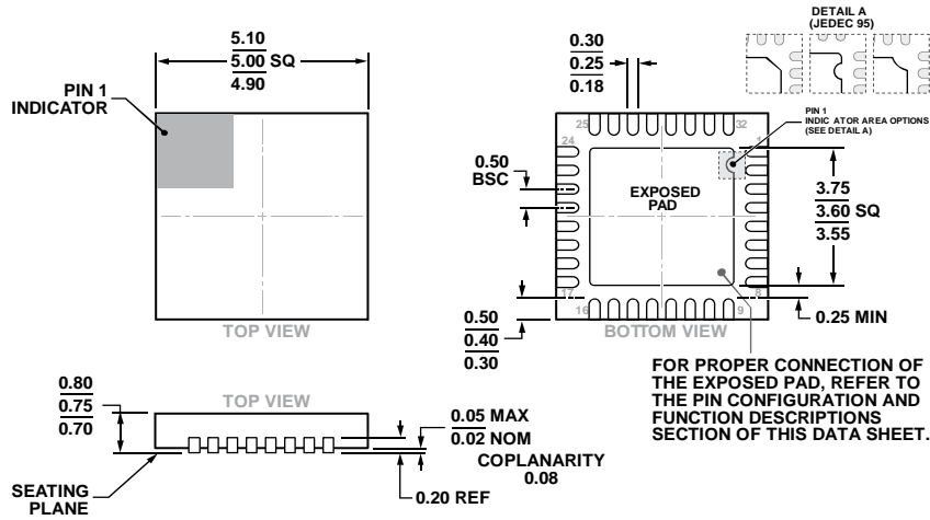
Figure 61. 32-Lead Lead Frame Chip Scale Package [LFCSP] 5 mm × 5 mm Body and 0.75 mm Package Height (CP-32-12) Dimensions shown in millimeters
